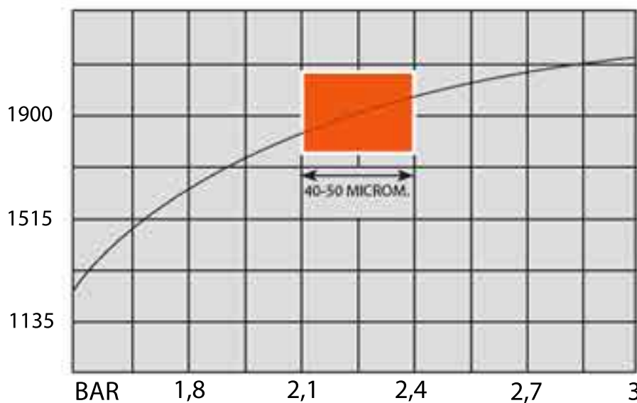
Liter/Minute 10" DESANDER CONE PERFORMANCE
