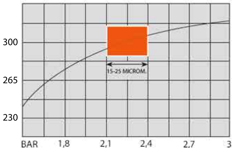
Liter/Minute 5" DESILTER CONE PERFORMANCE
